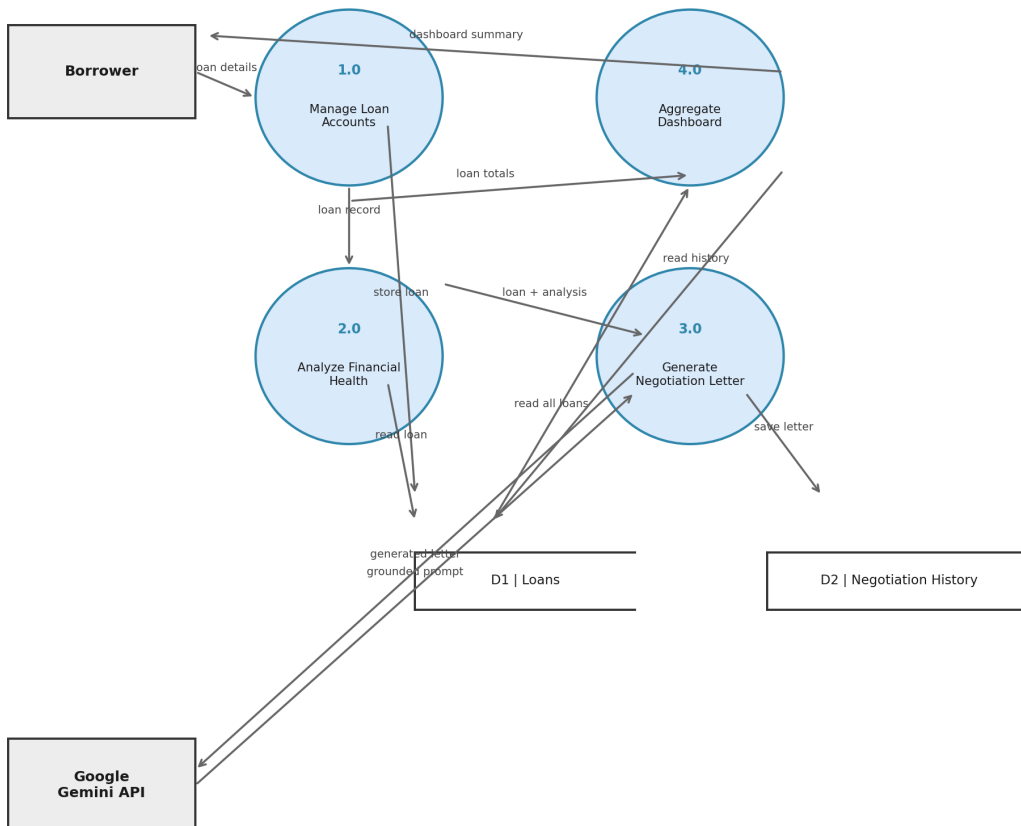
Data Flow Diagram (Level 1) — AI-Powered Debt Relief & Financial Recovery Platform
